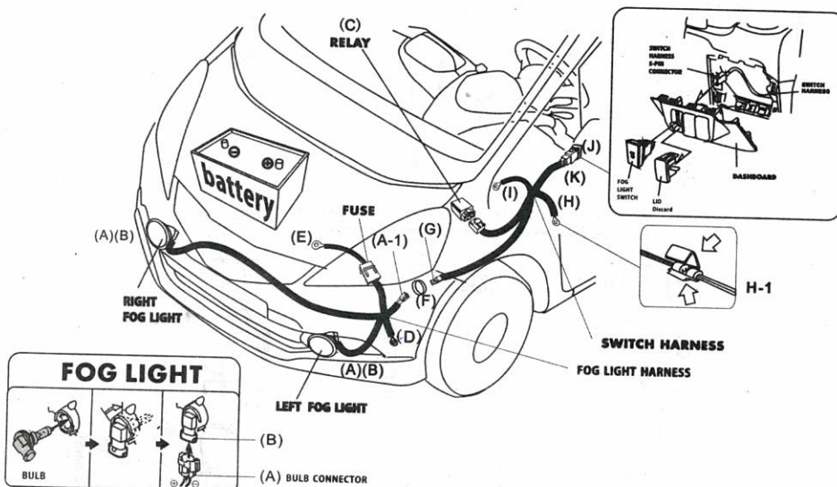
Illustration of Fog Light Wiring Kit Installation On Vehicle
